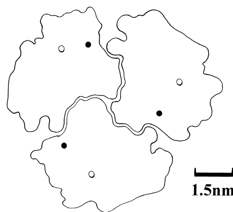
Fig. 3 Schematic diagram showing the proximity of Cys-144 to the dimer-dimer interface. The side chain SH group of Cys-144 (filled circles) which becomes accessible to modification by DTNB in the D165H mutant is shown in each subunit lying close to the dimer-dimer interface. The side chain SH group of the other cysteine residue which is accessible to DTNB modification in both wild-type and D165H (Cys-320) is shown near the centre of each subunit (open circles)
